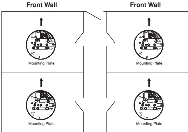
Fig.9 Orientate all mounting plates in the same direction
